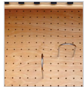
Versatile peg board with (7) metal dividers
